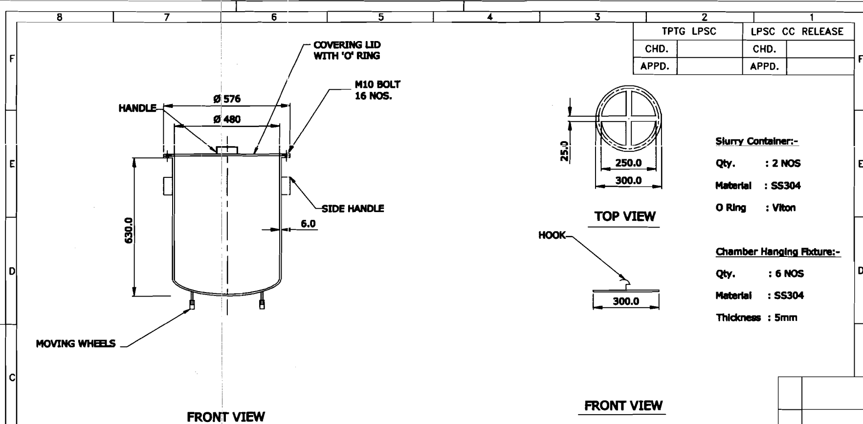
CHAMBER HANGING FIXTURE
